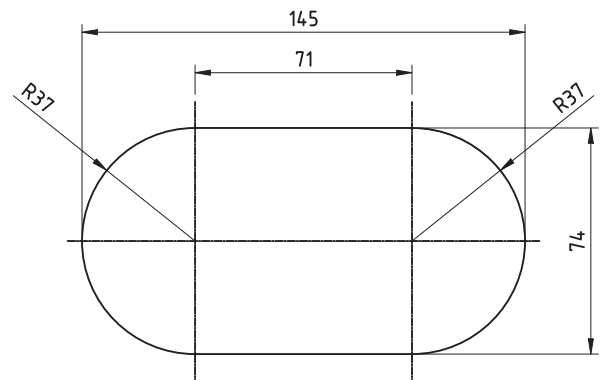
CUTTING HOLE
